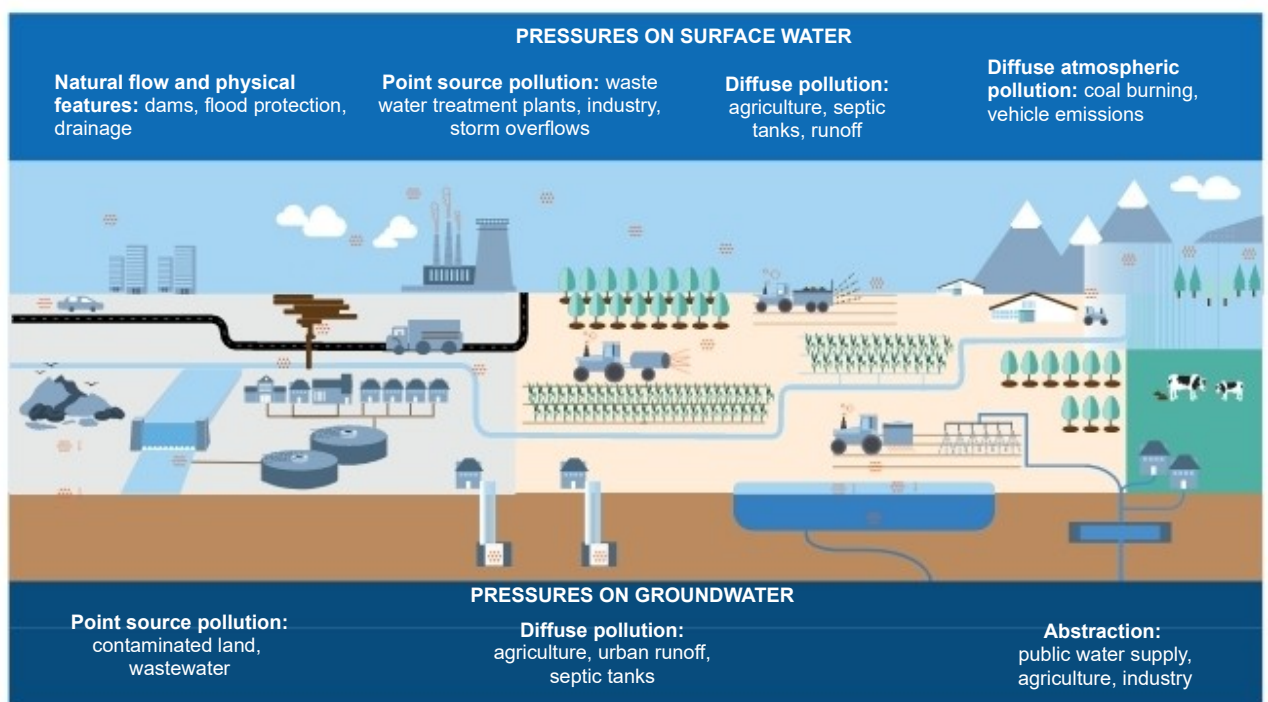
Figure 4.4 Pressures on surface and groundwater
